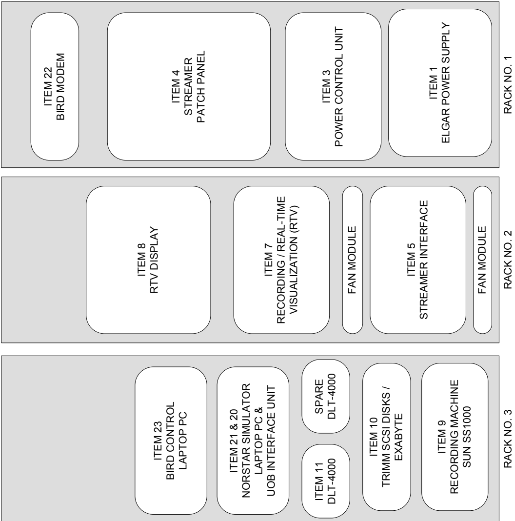
19" RACK FRONT VIEW
