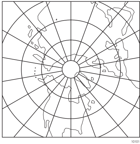
Figure 4.5. Stereographic
