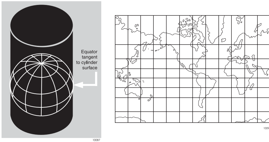
Figure 4.2. Mercator
