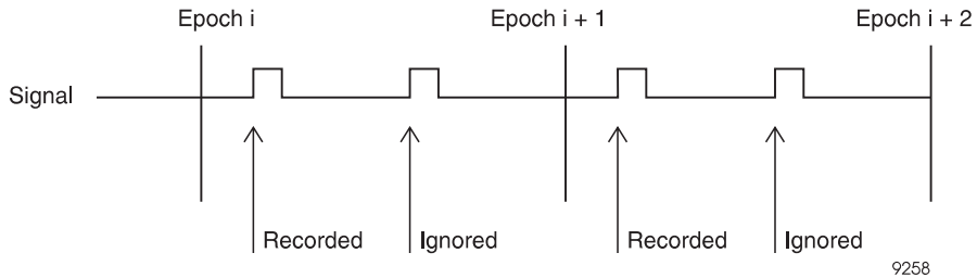
Figure 3.1. GPS Epochs
