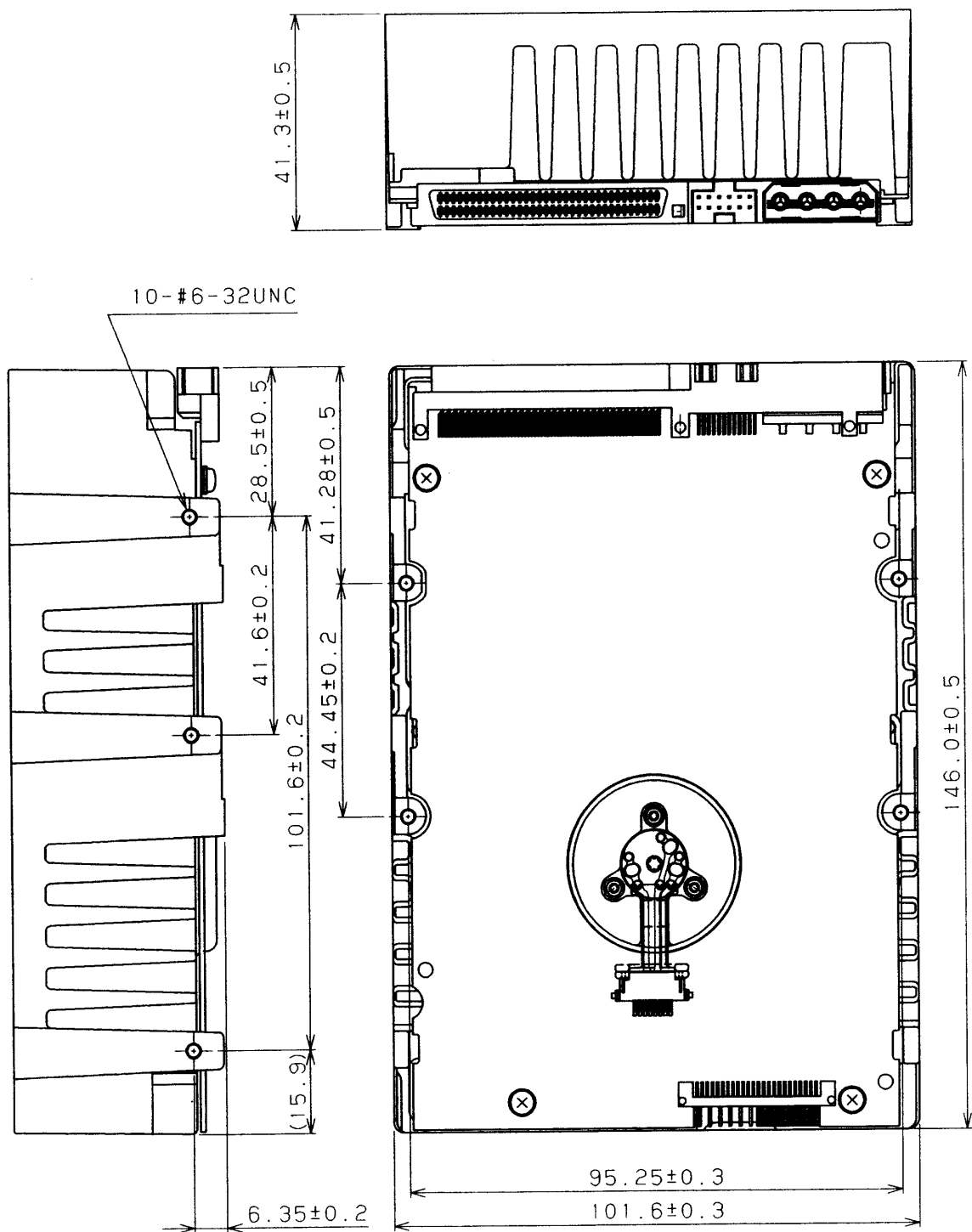
Figure 4.2 External dimensions (MAD33xxLP, MAF33xxLP)
