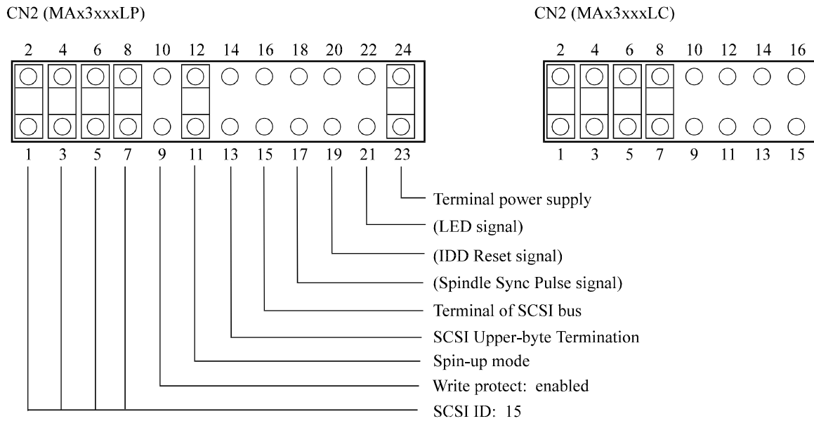
Figure 5.3 Setting terminals (MAX3xxxxx)
