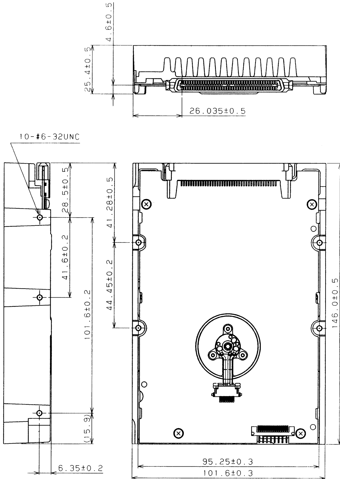
Figure 4.3 External dimensions (MAE31xxLC, MAE30xxLC)
