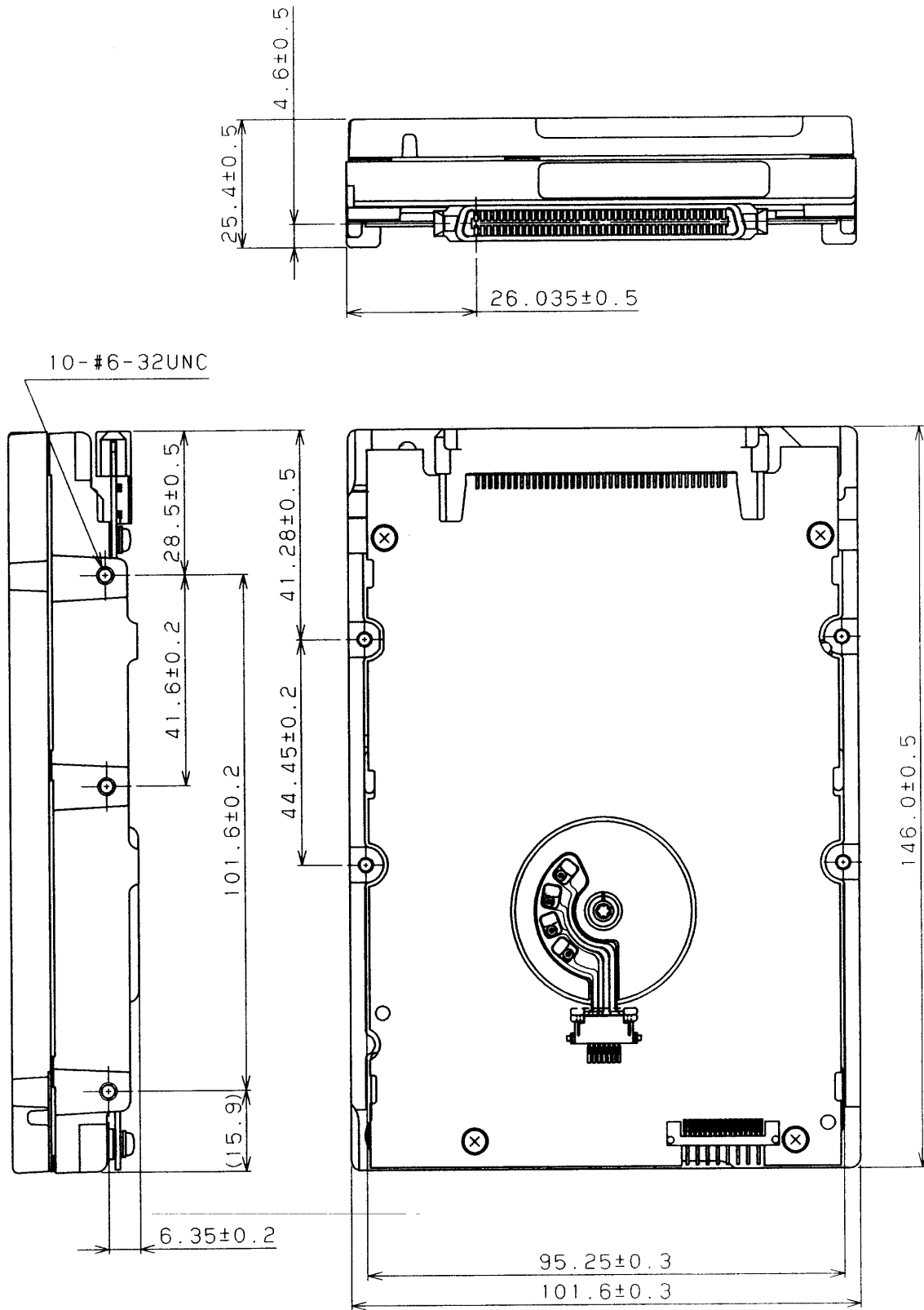
Figure 4.5 External dimensions (MAG31xxLC, MAG30xxLC)
