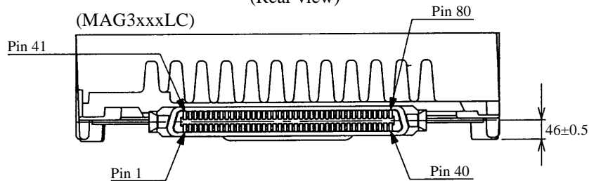
Figure A.1 Locations of connectors and setting terminals (Mx3xxxLC: SCA2 type LVD 16-bit SCSI)
