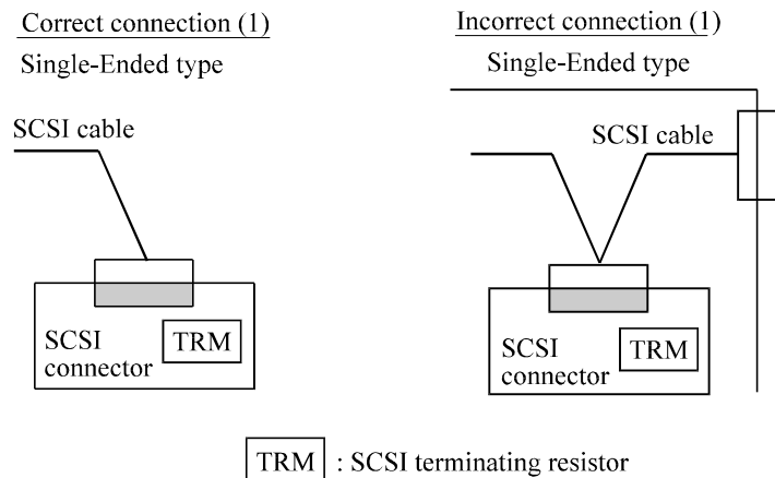
Figure 4.29 SCSI cable termination
