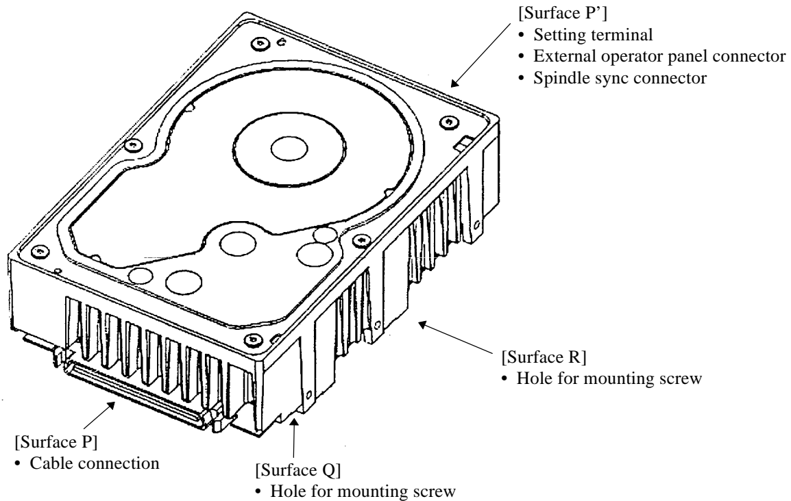
Figure 4.11 Service clearance area
