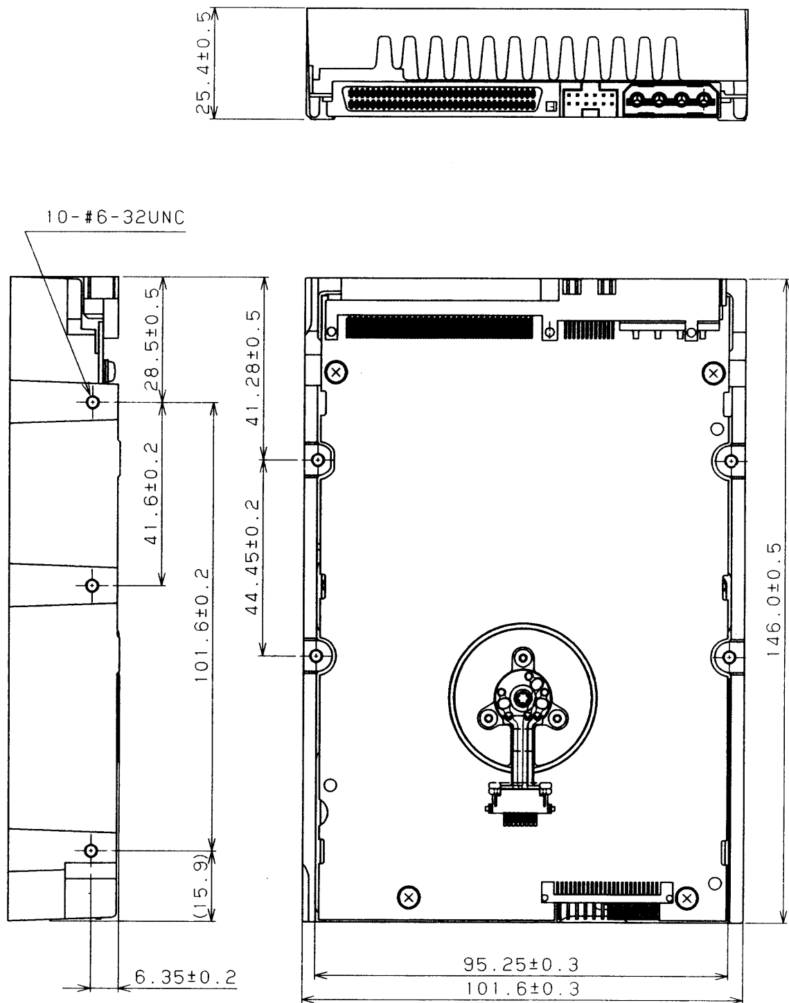
Figure 4.4 External dimensions (MAE31xxLP, MAE30xxLP)
