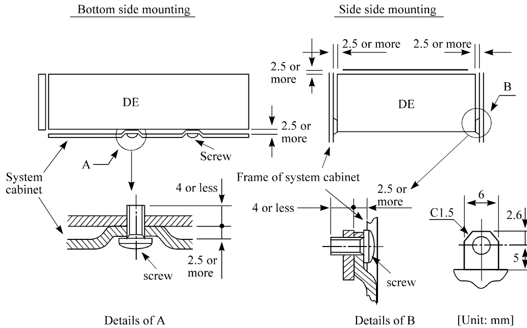
Figure 4.8 Mounting frame structure
