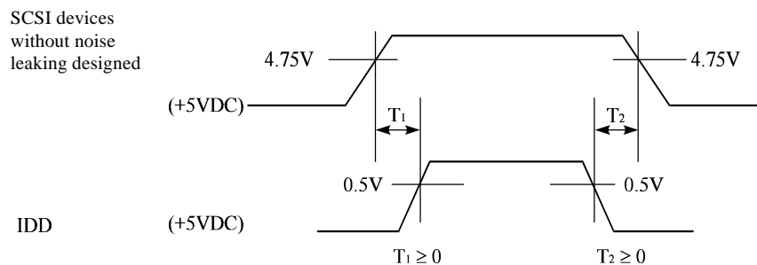
Figure 4.16 Power on/off sequence (3)
