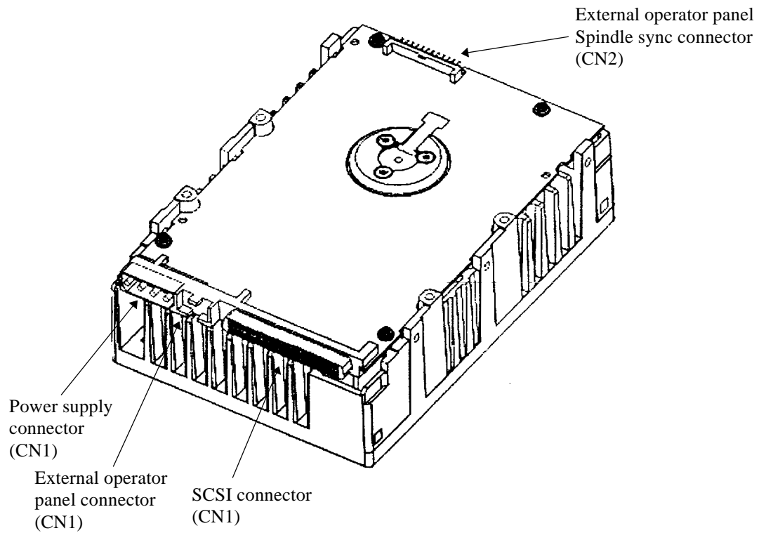
Figure 4.18 Connectors and terminals location (single-ended 16-bit SCSI)
