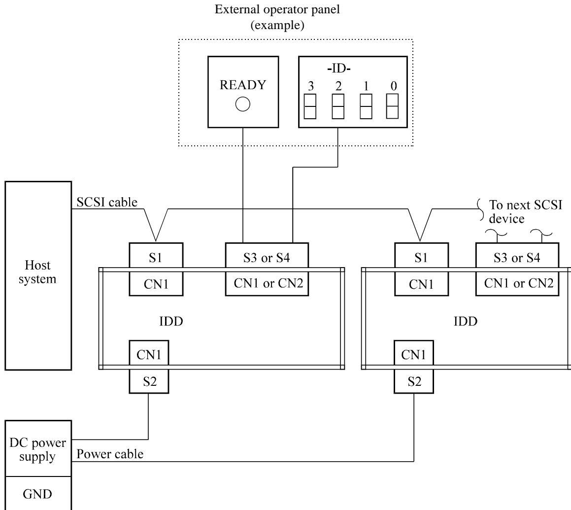
Figure 4.25 Cables connection (16-bit SCSI model)
