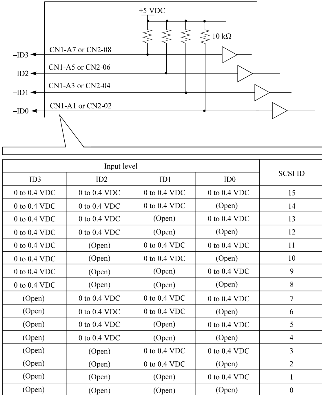
Figure 4.23 16-bit SCSI ID external input
