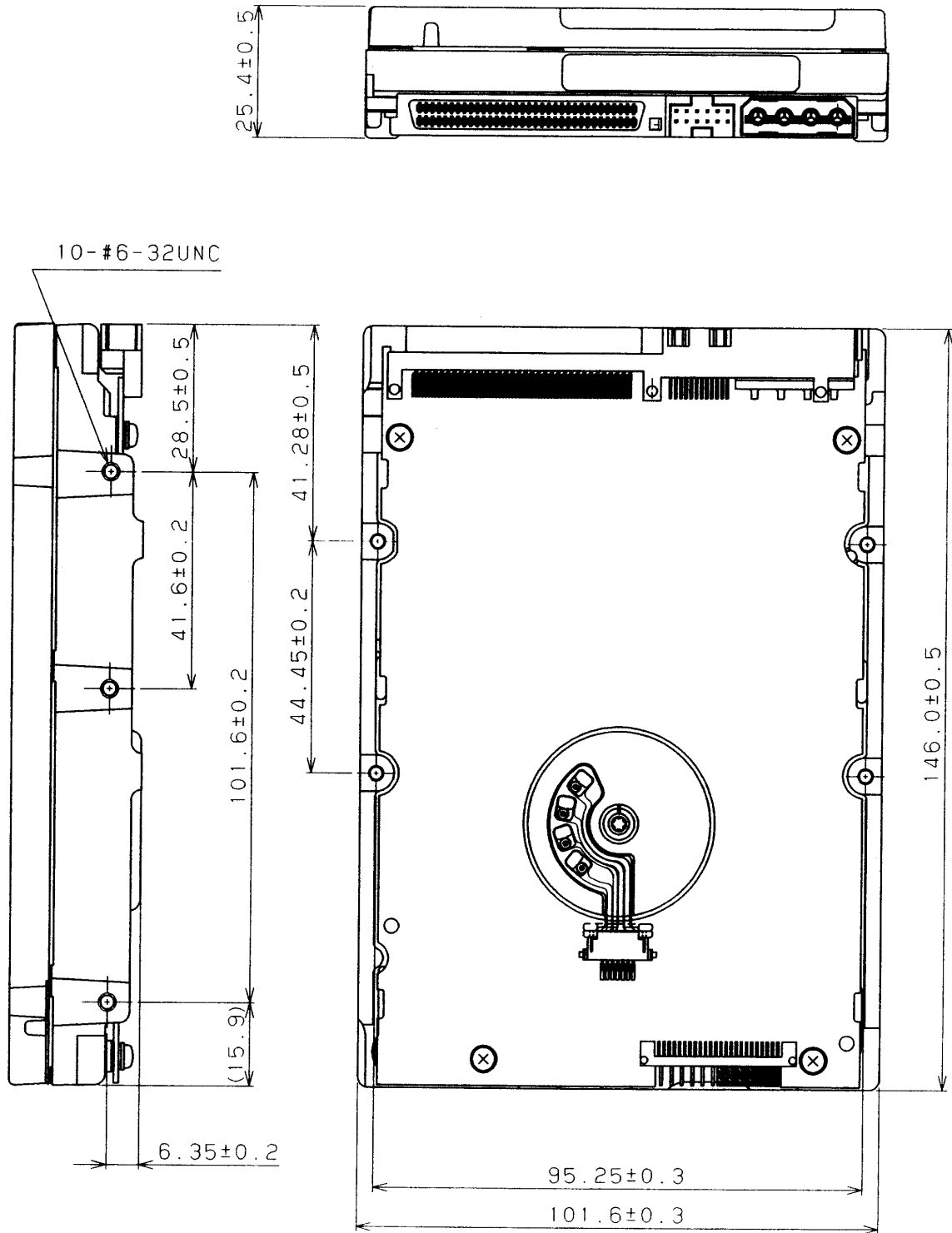
Figure 4.6 External dimensions (MAG31xxLP, MAG30xxLP)
