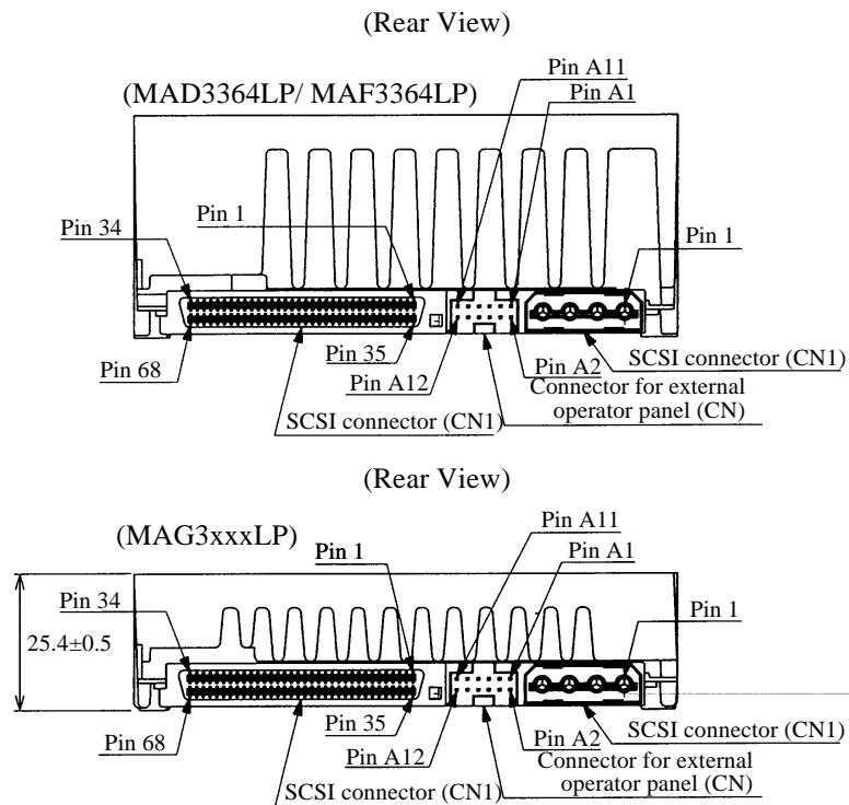
Figure A.2 Locations of connectors and setting terminals (Mx3xxxLP: 68 pin type LVD 16-bit SCSI)
