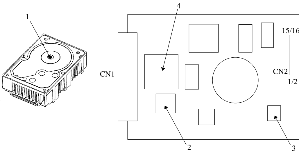
Figure 4.10 Surface temperature measurement points (MAD33xxxx, MAF33xxxx, MAE31xxxx, MAG31xxxx, MAE30xxxx, MAG30xxxx)
