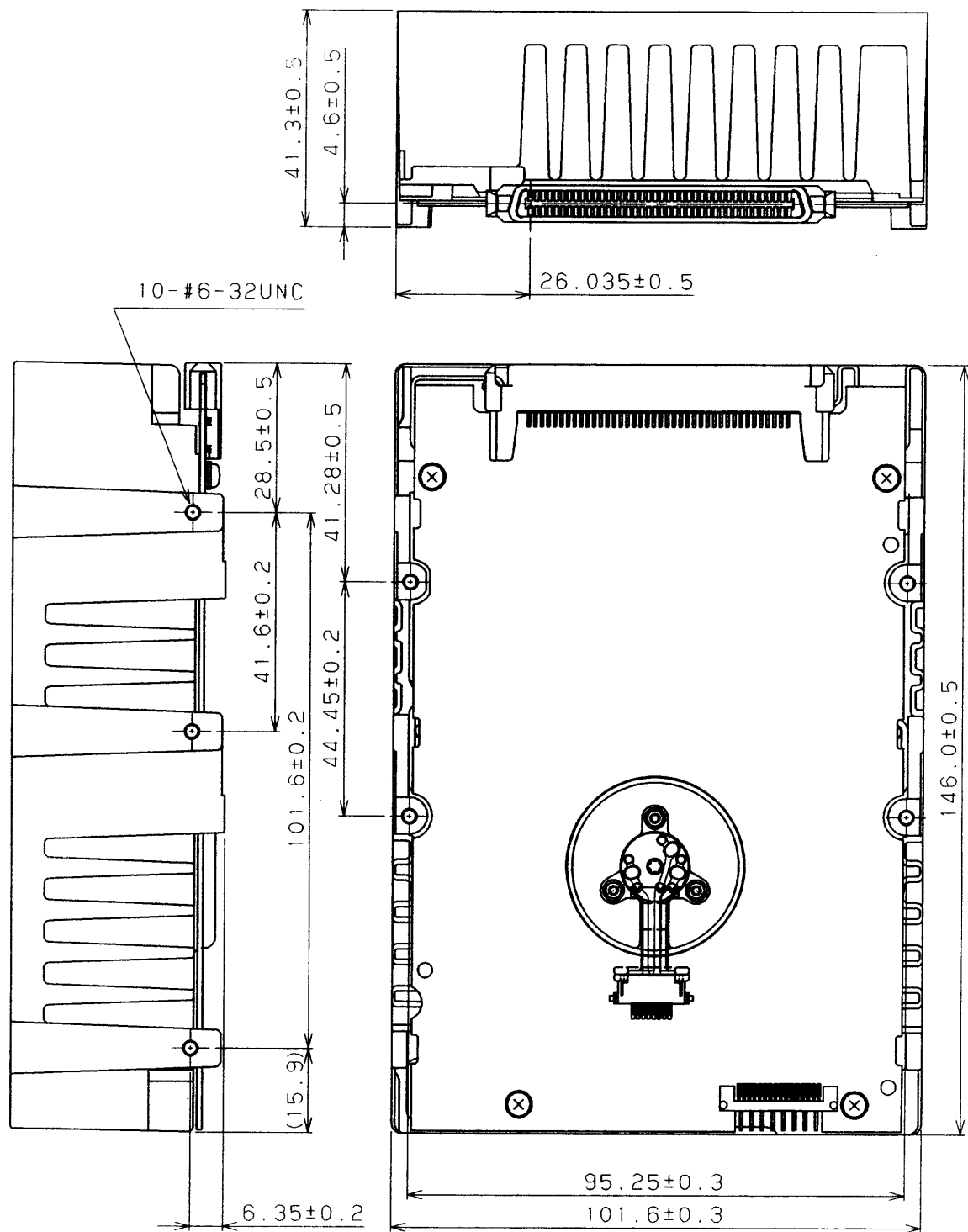
Figure 4.1 External dimensions (MAD33xxLC, MAF33xxLC)
