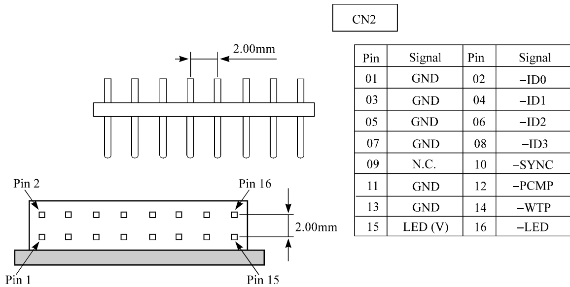
Figure 4.22 External operator panel connector (CN2)
