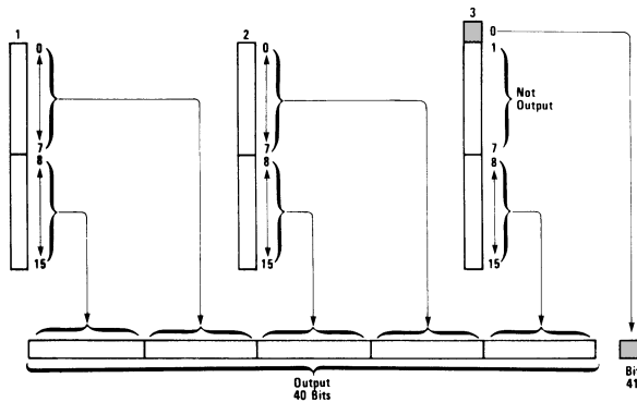
Figure 2. Output assembly in binary mode
