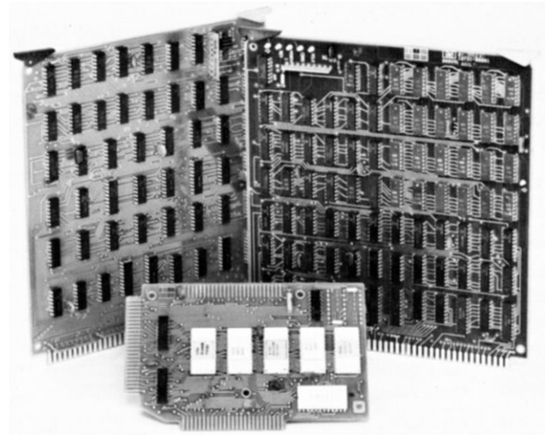
12976B and 003 Dynamic mapping system; firmware board (foreground) includes Fast Fortran processor instructions as well as dynamic mapping instructions
