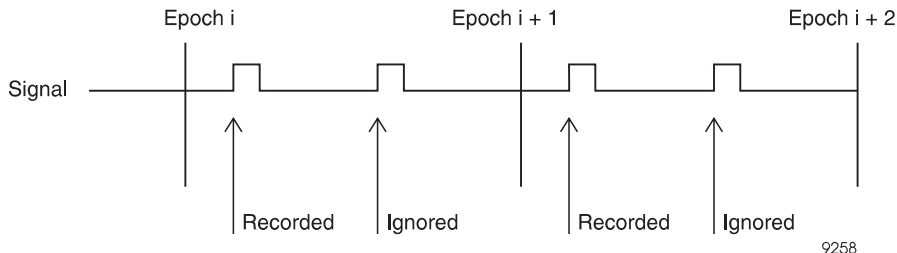
Figure 3.1. GPS Epochs
