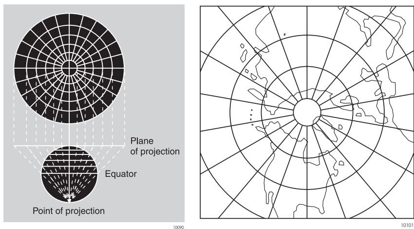
Figure 4.5. Stereographic
