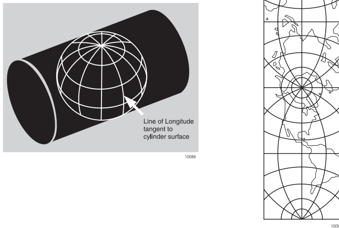
Figure 4.3. Transverse Mercator
