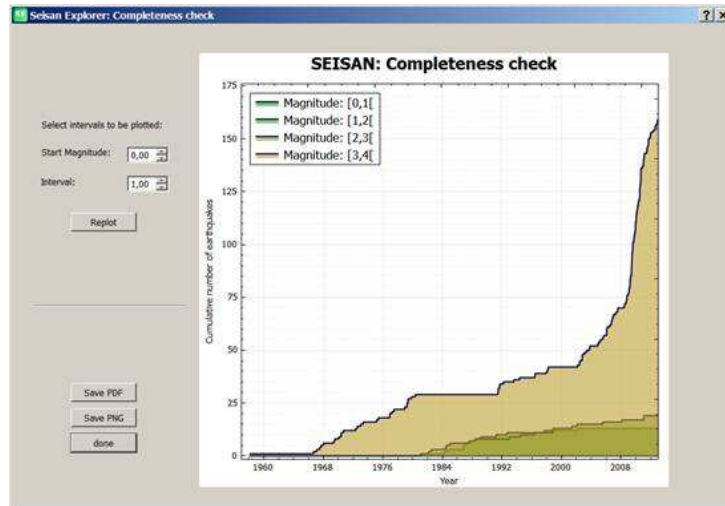
Figure 4.9: se-completeness
