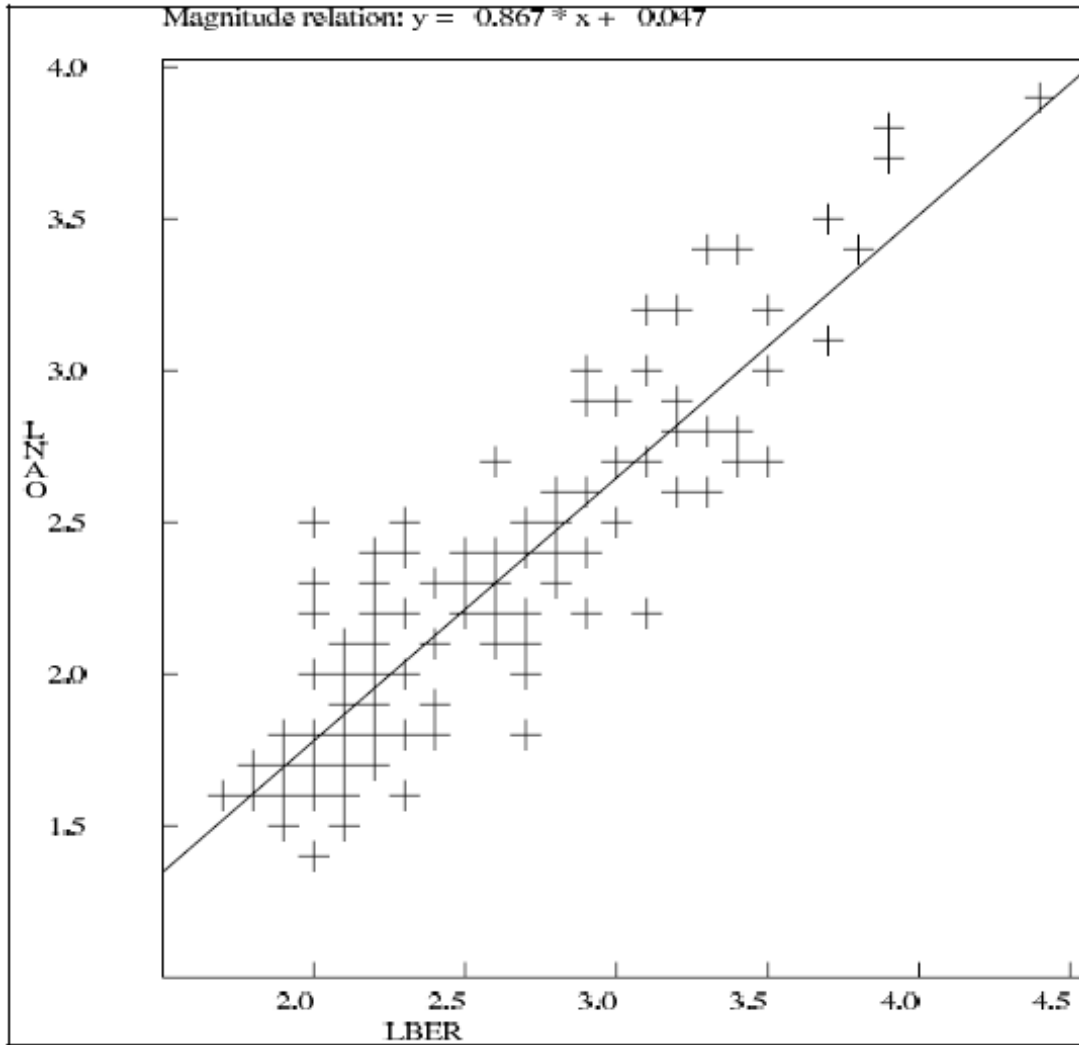
Figure 6.47: Example of using the MAG program. Relation between NOR SAR and Bergen local magnitudes.
