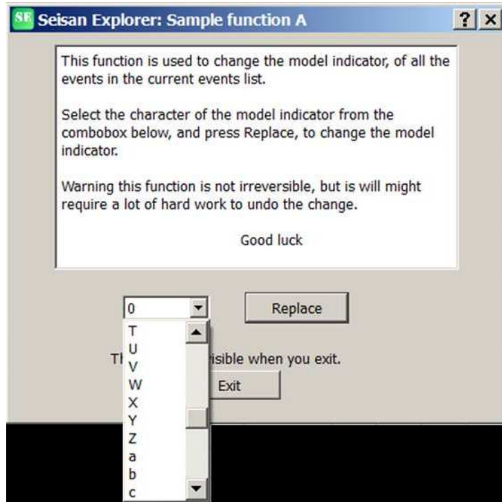
Figure 4.13: se-change-model-indicator
