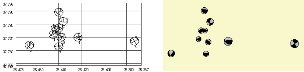
Figure 6.32: Plotting many fault plane solutions. Left: Using W-EMAP. Notice that the colors in the solutions are inverted compared to normal practice. Right: Using EPIMAP. The data for the two plots is the same.
