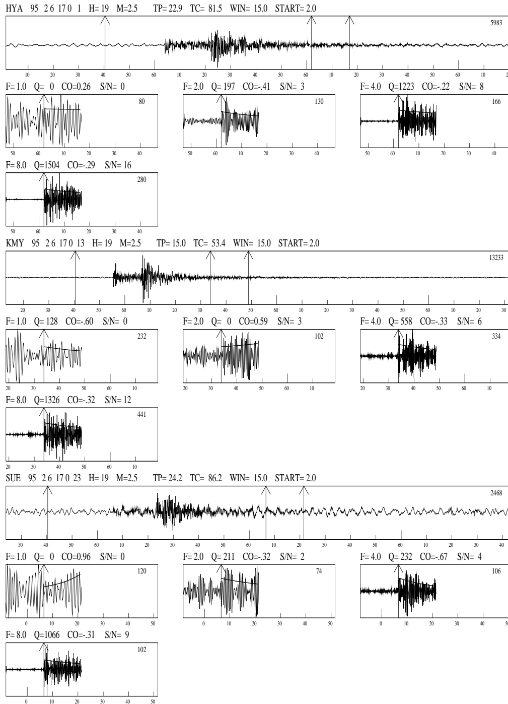
Figure 6.39: An example of a coda Q plot. On top is shown the original trace and below the filtered coda windows. Note that 15 secs of noise are shown in front of the selected filtered coda window. The first 5 secs of the noise shown is used for calculating the S/N ratio. On each filtered plot is given F: Center frequency, Q: Q-value, zero means no Q-value could be calculated, S/N: Signal to noise ratio.
