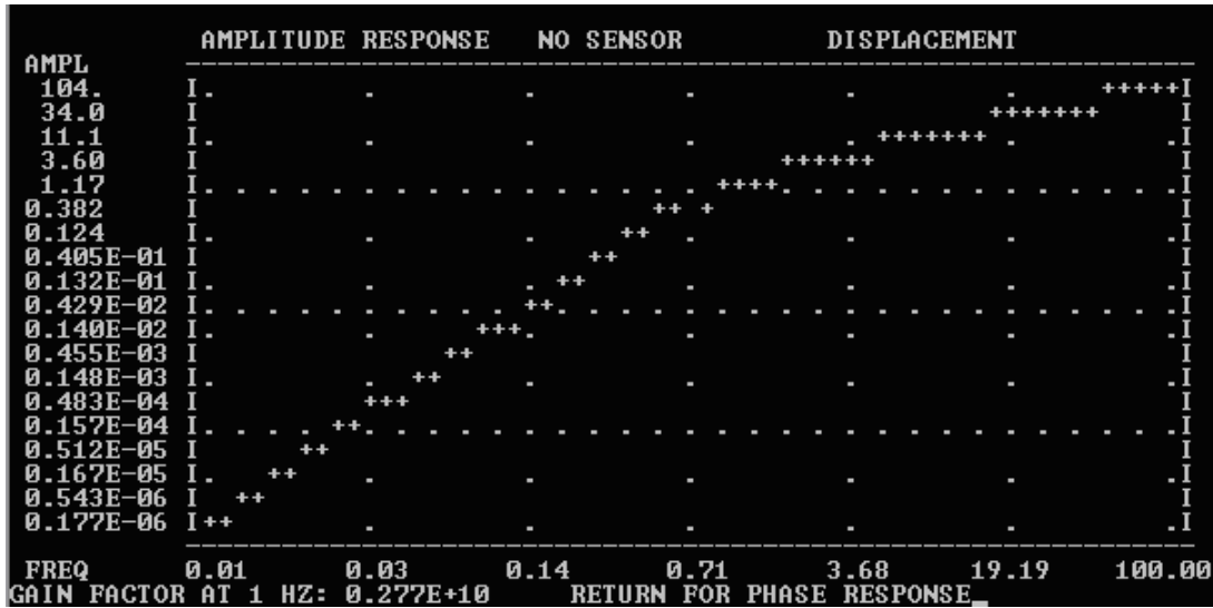
Figure 6.53: Making response file with poles and zeros.
