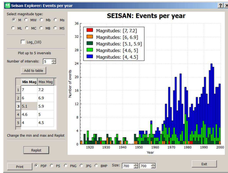
Figure 4.15: se-events-per-year
