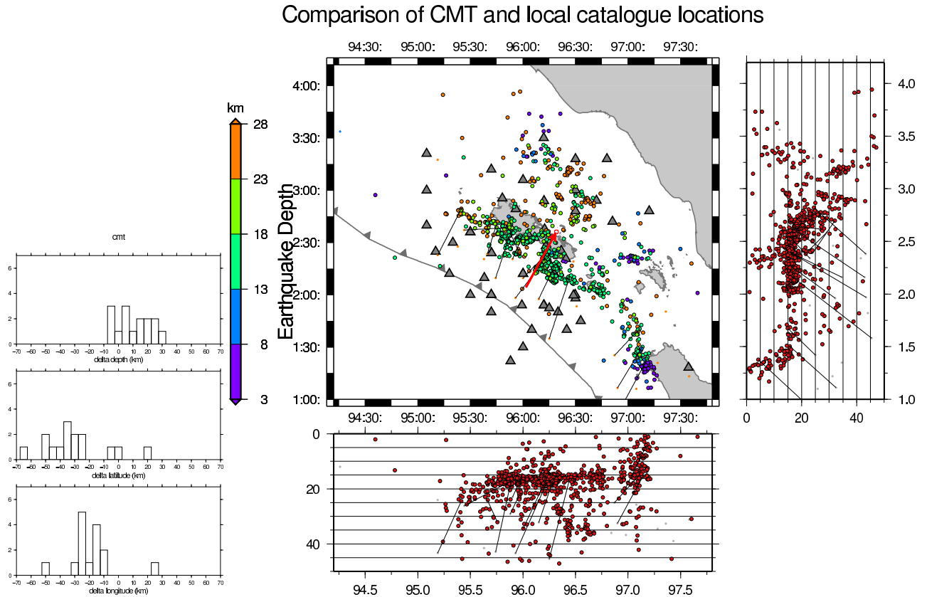
Figure 6.42: (Left) Histogram of the offsets between locations in the GCMT catalogue and a catalogue based on an OBS/land deployment offshore Northern Sumatra [Tilman et al., 2010], generated using the -d=xyz option and GMT pshistogram . (Right) Map and cross-sectional views. Large rimmed circles are events in the local catalogue, and small borderless circles are locations in the GCMT catalogue. Lines connect associated events (drawn using -d=gmt option and GMT psxy ). The red arrow points in the direction of the average shift between CMT and local locations, with the little red circle showing the formal uncertainty of the average shift vector (generated using -d=bias option and GMT psve1o ). Its absolute size is only meaningful if the formal errors of the contributing locations are all realistic. The plots show the tendency of CMT centroids in subduction zones to be located seaward off and deeper than their actual location.
