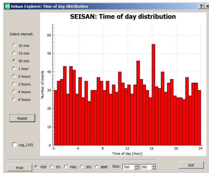
Figure 4.16: se-time-of-day
