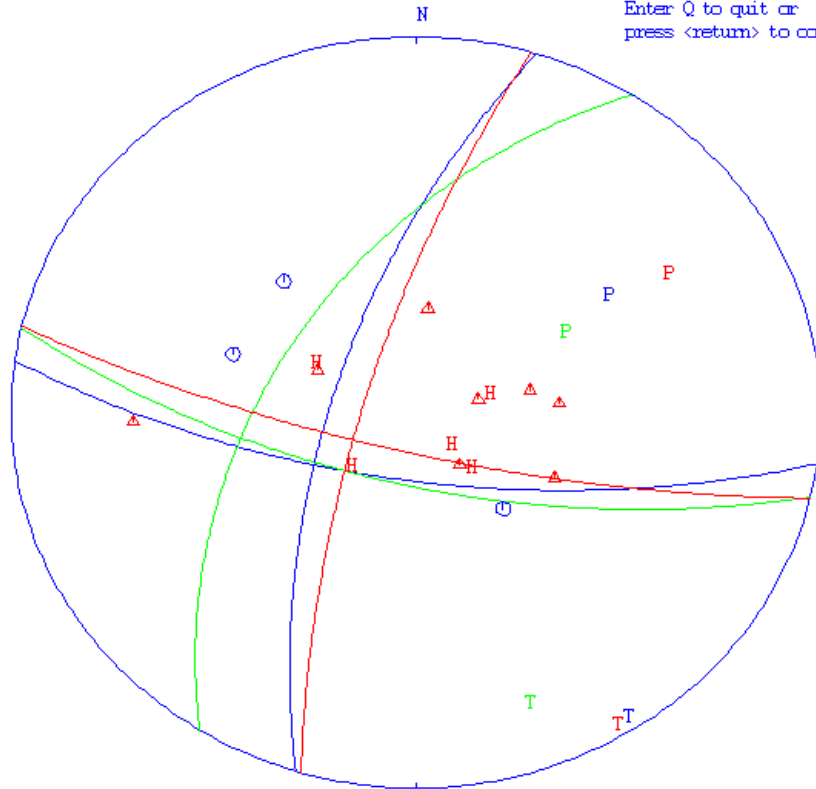
Figure 6.30: Compare fault plane solutions from different programs. For explanation of symbols, see FOCMEC.
