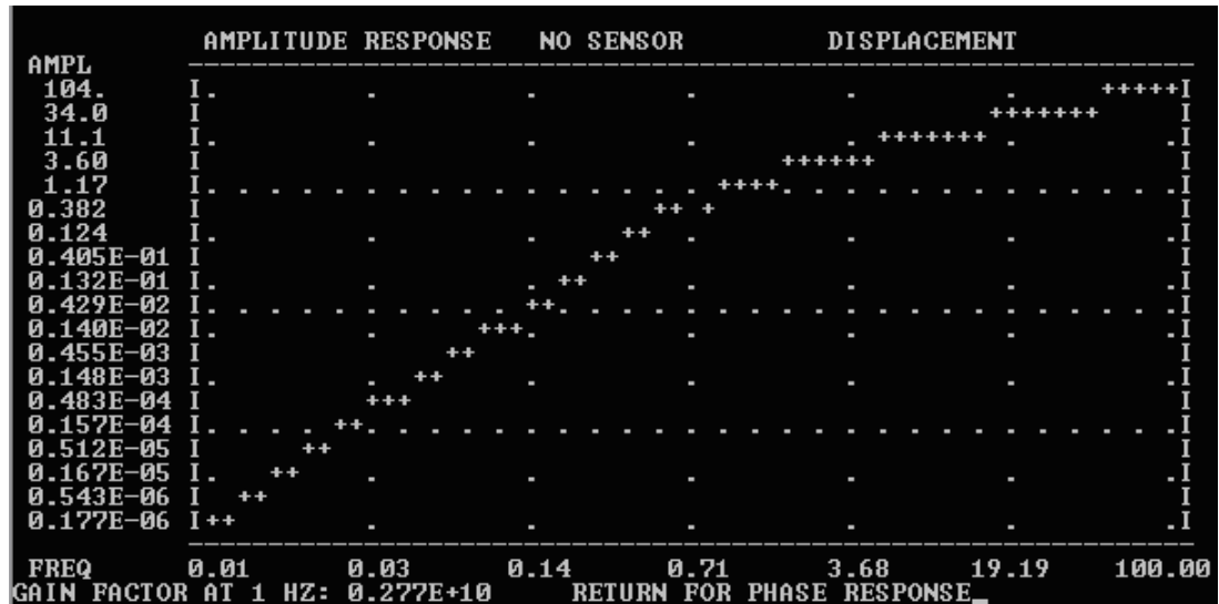
Figure 6.53: Making response file with poles and zeros.
