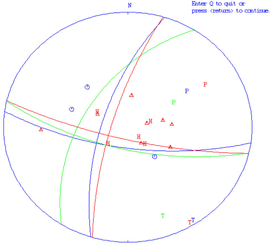
Figure 6.30: Compare fault plane solutions from different programs. For explanation of symbols, see FOCMEC.
