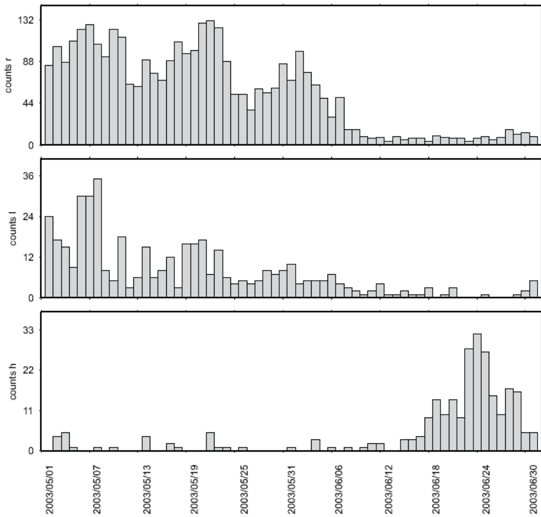
Figure 6.49: Bar diagrams showing distribution of events of different subclasses over time.
