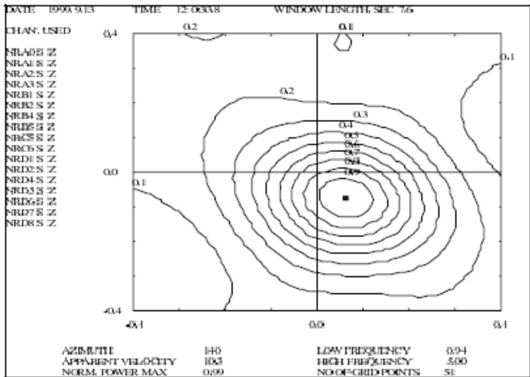
Figure 6.51: Output from the FK program. Contours and values are the normalized maximum power.
