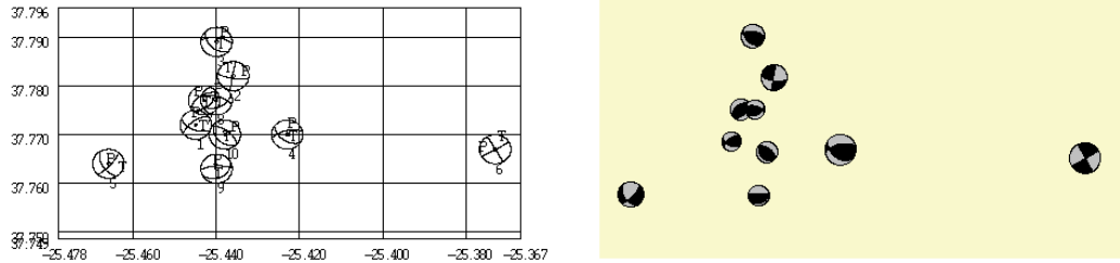
Figure 6.32: Plotting many fault plane solutions. Left: Using WEMAP. Notice that the colors in the solutions are inverted compared to normal practice. Right: Using EPIMAP. The data for the two plots is the same.
