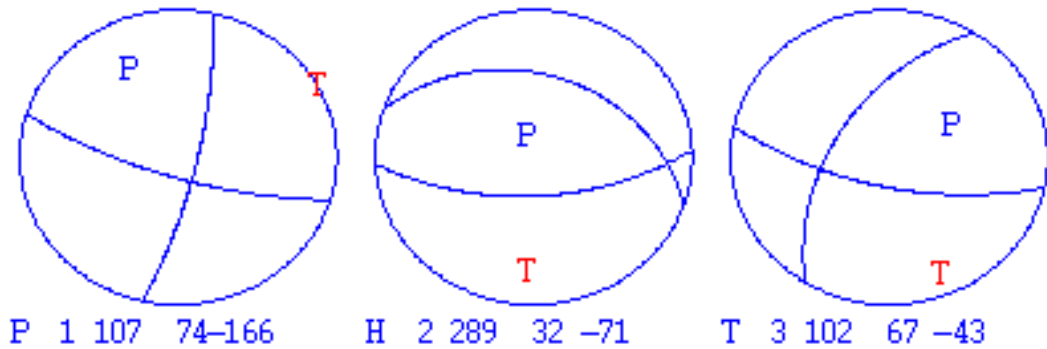
Figure 6.29: Using FOC to plot solutions from fps.out . The program used for each solution is given with a one letter code: P: PINV, F: FOCMEC, H: HASH and T: FPFIT.
