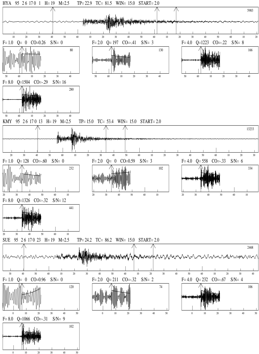
Figure 6.39: An example of a coda Q plot. On top is shown the original trace and below the filtered coda windows. Note that 15 secs of noise are shown in front of the selected filtered coda window. The first 5 secs of the noise shown is used for calculating the S/N ratio. On each filtered plot is given F: Center frequency, Q: Q-value, zero means no Q-value could be calculated, S/N: Signal to noise ratio.
