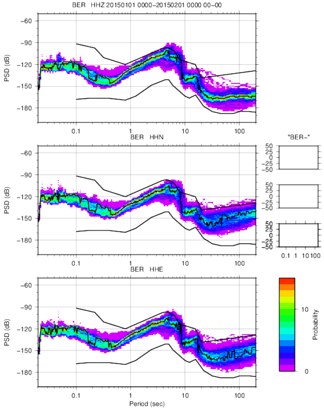
Figure 6.21: Example of plot created using CONNOI and EVANOI. The plot shows noise PDFs for station BER for three components in January 2015.
