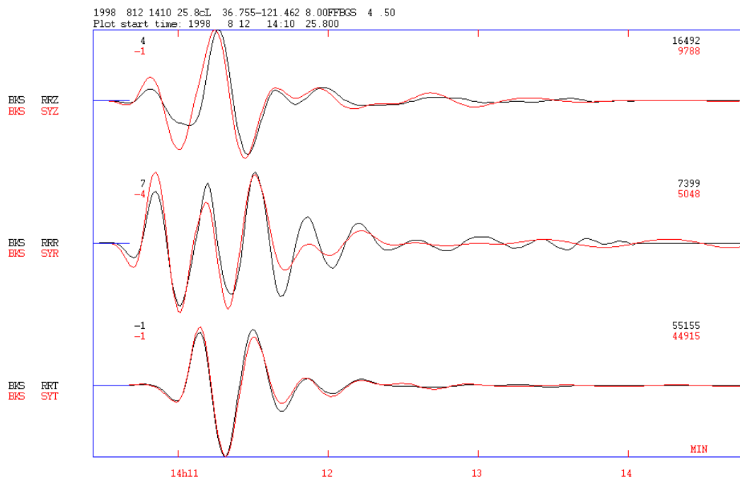
Figure 6.37: Same data as shown in previous figure but only for station BKS. The data is now auto scaled. The fit on all channels is quite good. Notice the small amplitude of the radial component.
