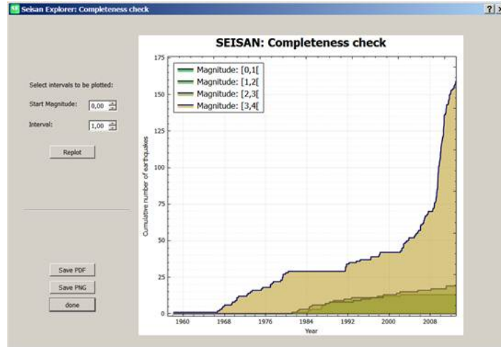
Figure 4.9: se-completeness
