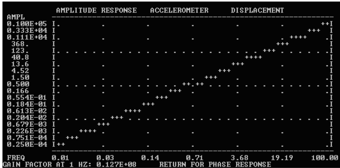
Figure 6.54: Making response file for an accelerometer with parameters.
