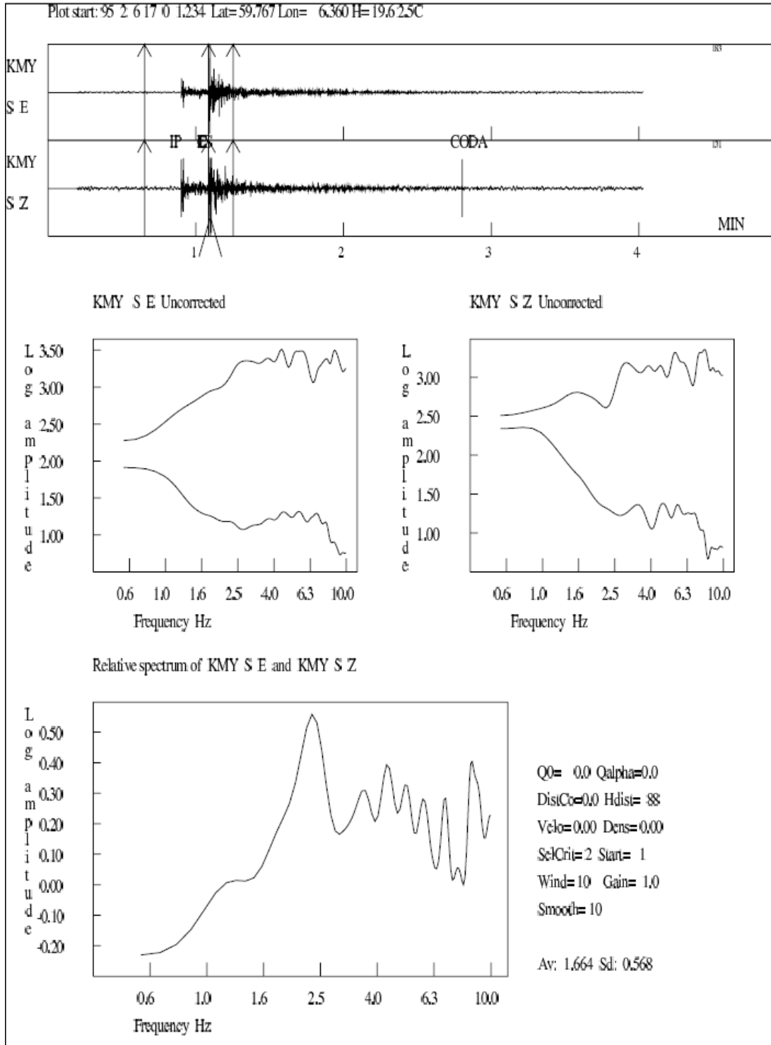
Figure 6.45: An example of using the SPEC program. On top the original traces are shown with windows chosen, in the middle the spectra of each channel and at the bottom, the relative spectrum. Lower right shows the input parameters used. In some cases ( \kappa and Q ) the values calculated for this case are also shown.
