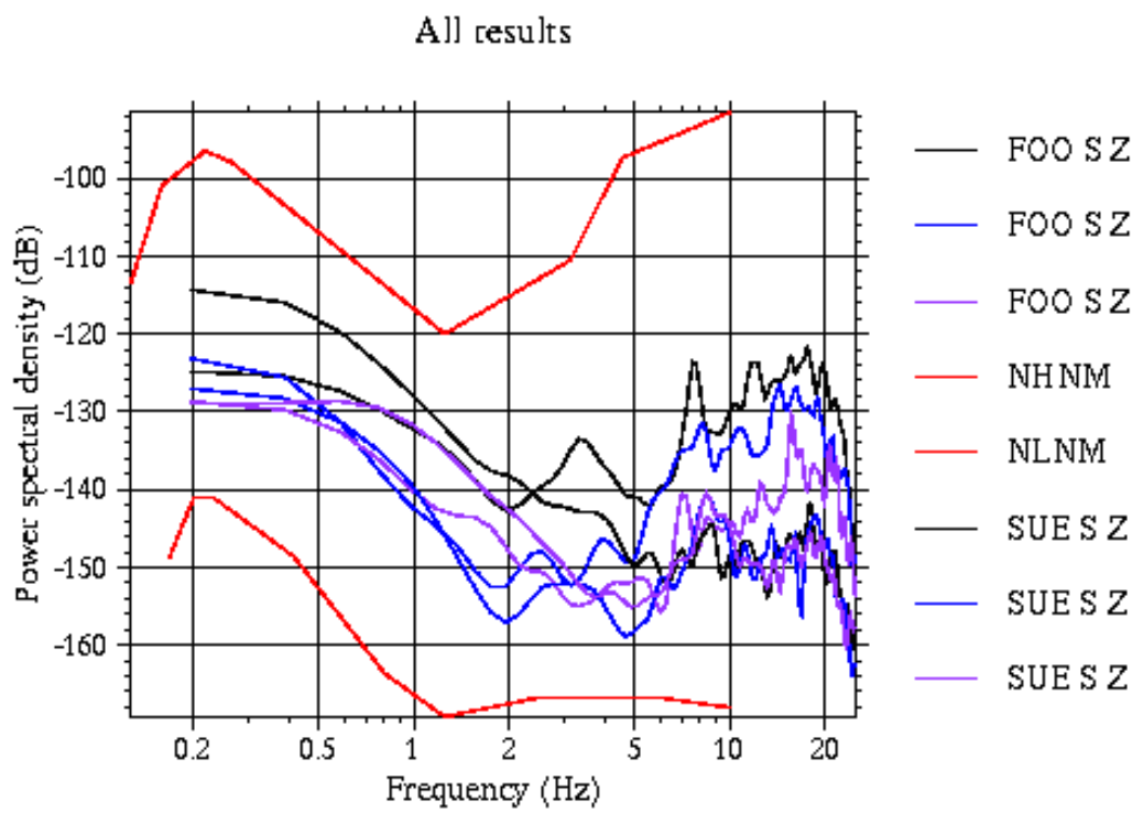
Figure 6.46: An example of a GMT plot. The figure shows an example of making noise spectra of several traces.
