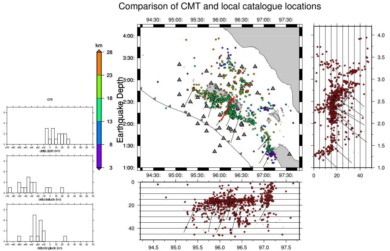
Figure 6.42: (Left) Histogram of the offsets between locations in the GCMT catalogue and a catalogue based on an OBS/land deployment offshore Northern Sumatra [Tilmann et al., 2010], generated using the -d=xyz option and GMT pshistogram . (Right) Map and cross-sectional views. Large rimmed circles are events in the local catalogue, and small borderless circles are locations in the GCMT catalogue. Lines connect associated events (drawn using -d=gmt option and GMT psxy ). The red arrow points in the direction of the average shift between CMT and local locations, with the little red circle showing the formal uncertainty of the average shift vector (generated using -d=bias option and GMT psvelo ). Its absolute size is only meaningful if the formal errors of the contributing locations are all realistic. The plots show the tendency of CMT centroids in subduction zones to be located seaward off and deeper than their actual location.
