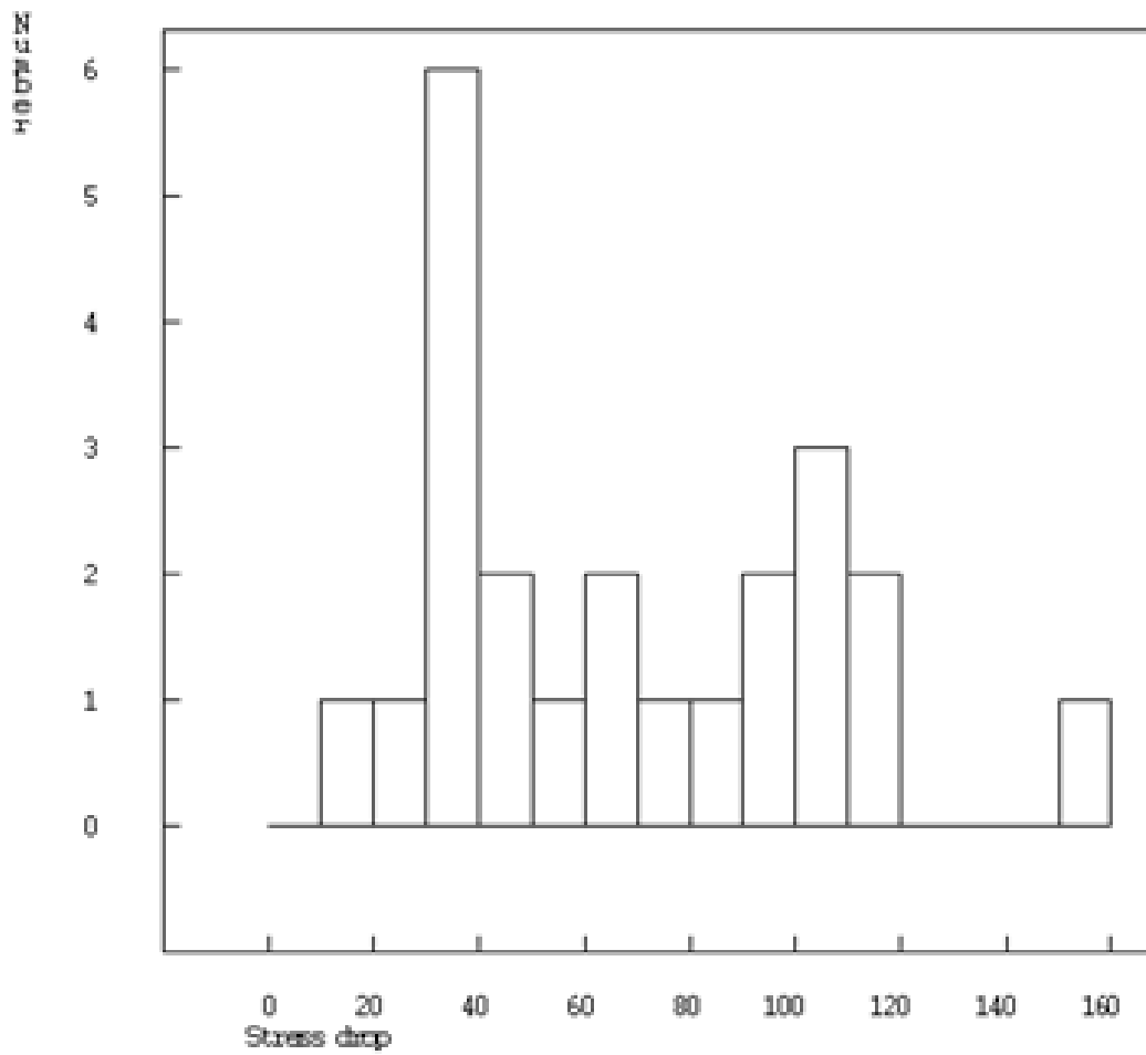
Figure 6.26: Histogram of stress drops.
