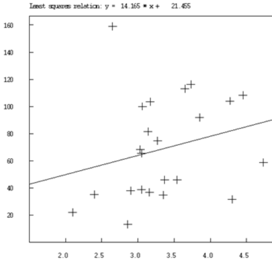
Figure 6.25: Stress drop versus Mw for 23 events.
