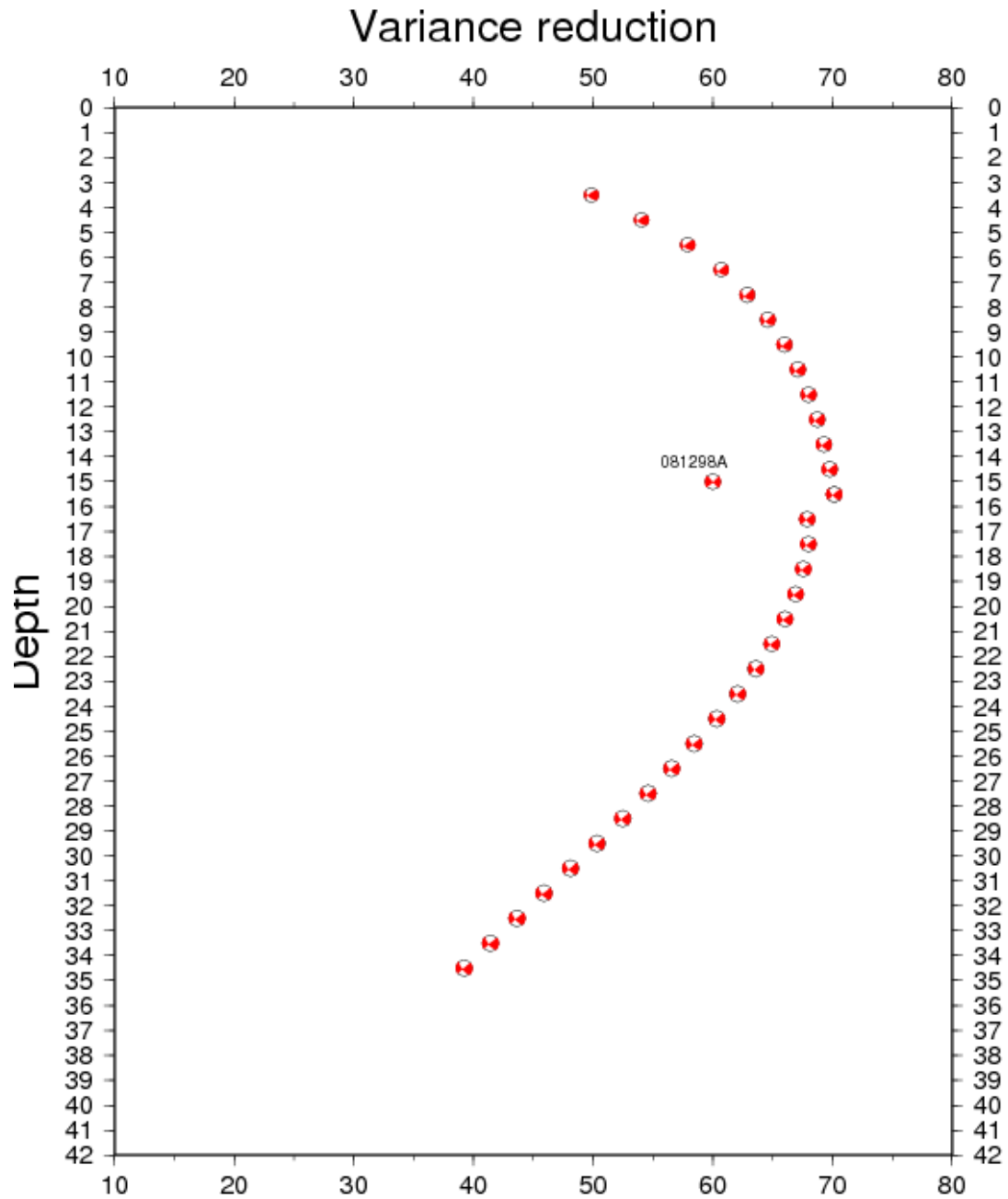
Figure 6.38: The double couple part of the moment tensor solution shown with respect to the variance reduction at different depths. The GCMT solution is also shown with arbitrary variance reduction. This figure was made with the GMT program psmeca , see text.
