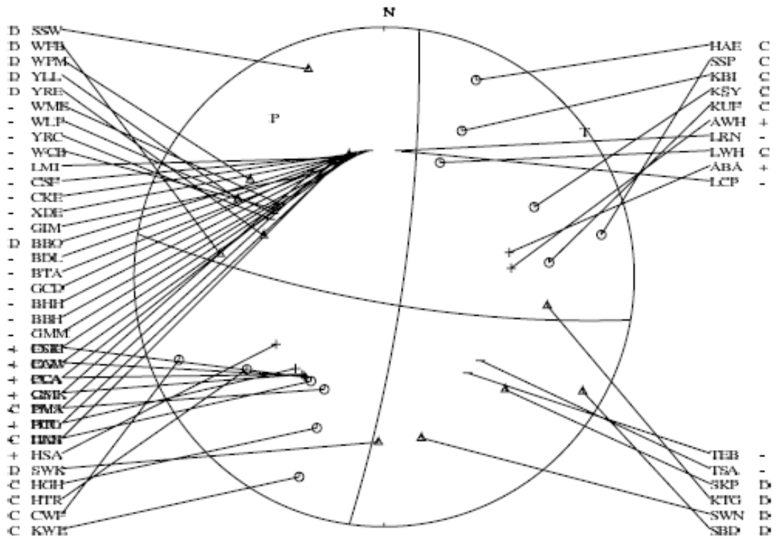
Figure 6.28: Top: An example of a fault plane solution plot. Symbols are explained in the text. Bottom: A fault plane solution also showing the stations with corresponding polarities.
