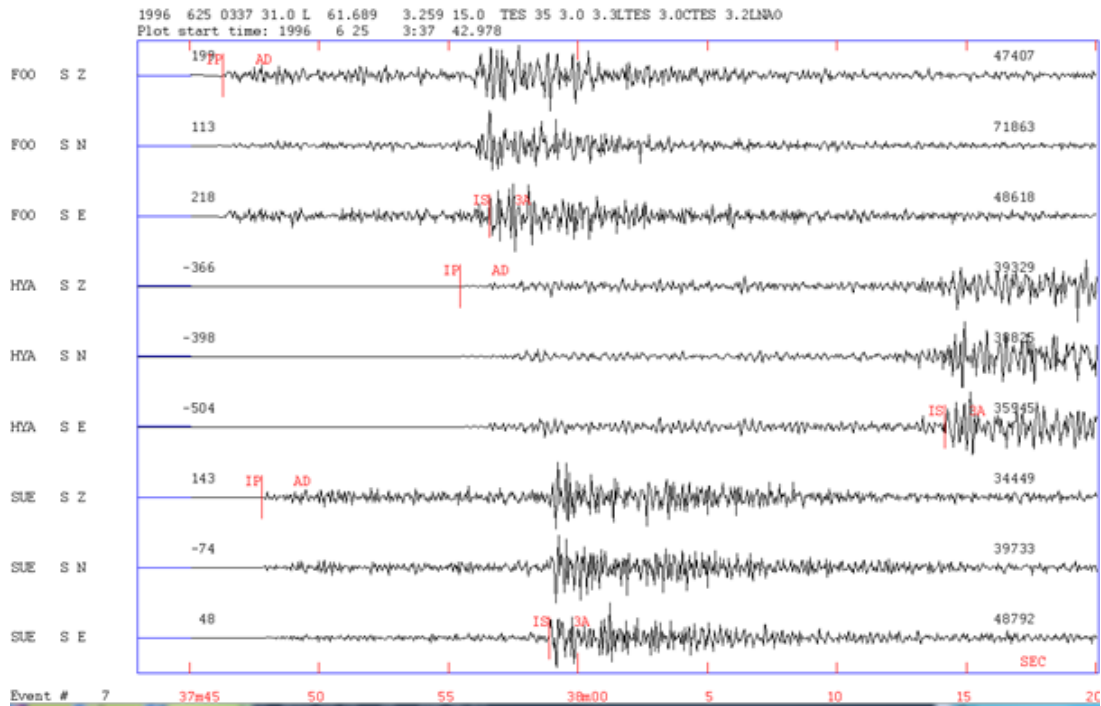
Figure 6.24: Examples of automatic picks on a "good" event.
