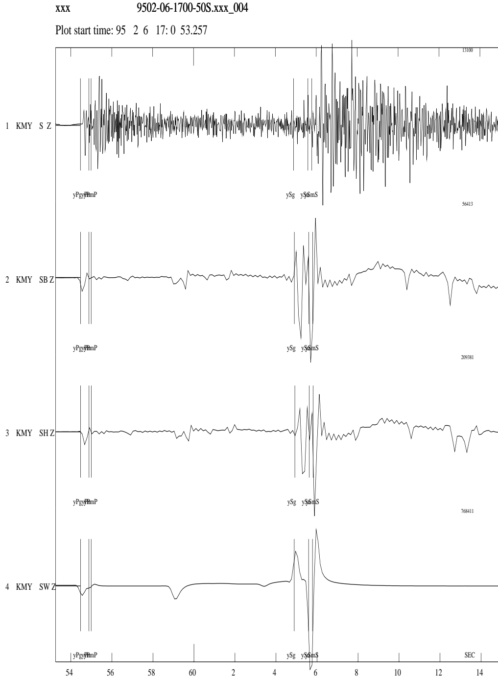
Figure 6.43: An example of synthetic seismograms using Bouchon(2), Herrmann (3) and WKBJ (4). The original seismogram is shown in channel 1. All synthetics are displacement. Also shown are the theoretical travel times calculated by WKBJ.
