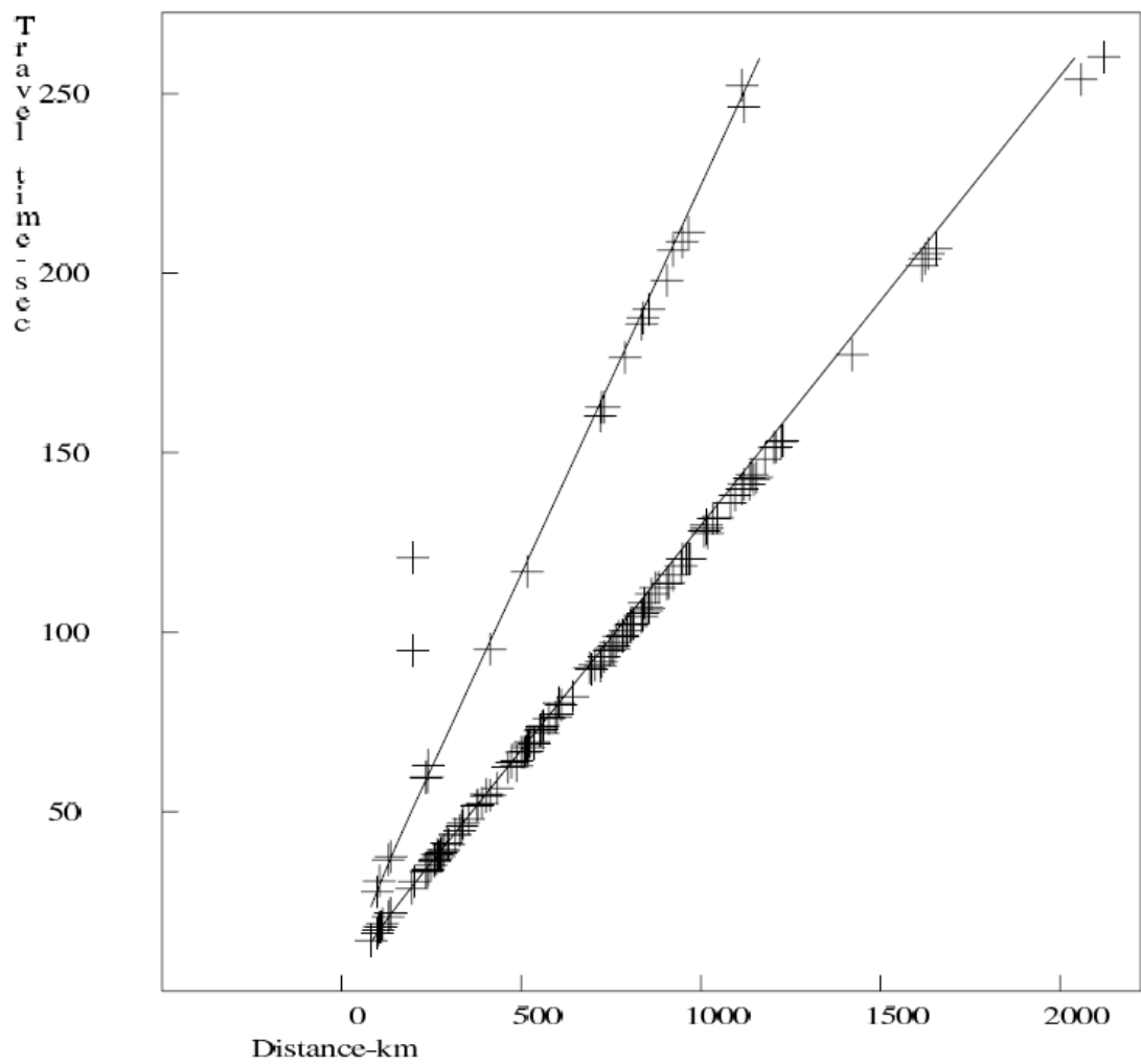
Figure 6.44: Example of travel time plot. Both P and S observed travel times are plotted with "+" symbol. Calculated times are shown by the solid lines, the lower one gives the first P arrivals, the upper line gives first S arrivals. The two outliers are observations from a station with incorrect timing.
