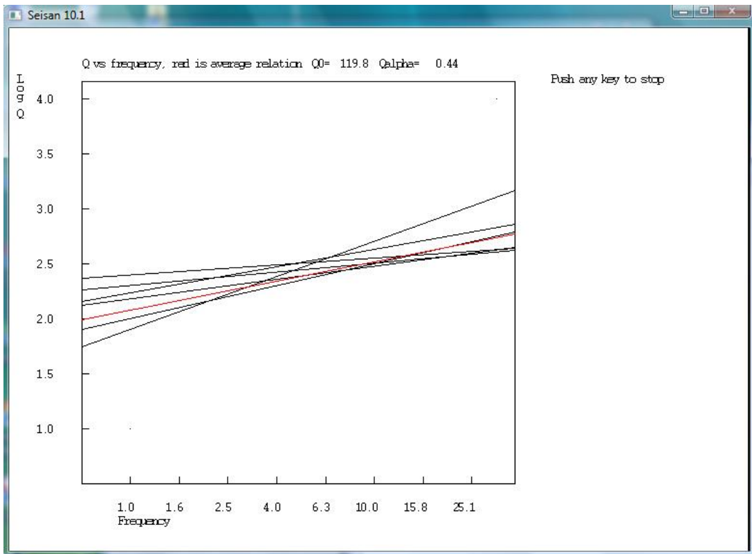
Figure 6.41: Figure AVQ: The figure shows the Q-relations to be averaged and the average Q-relation (red).
