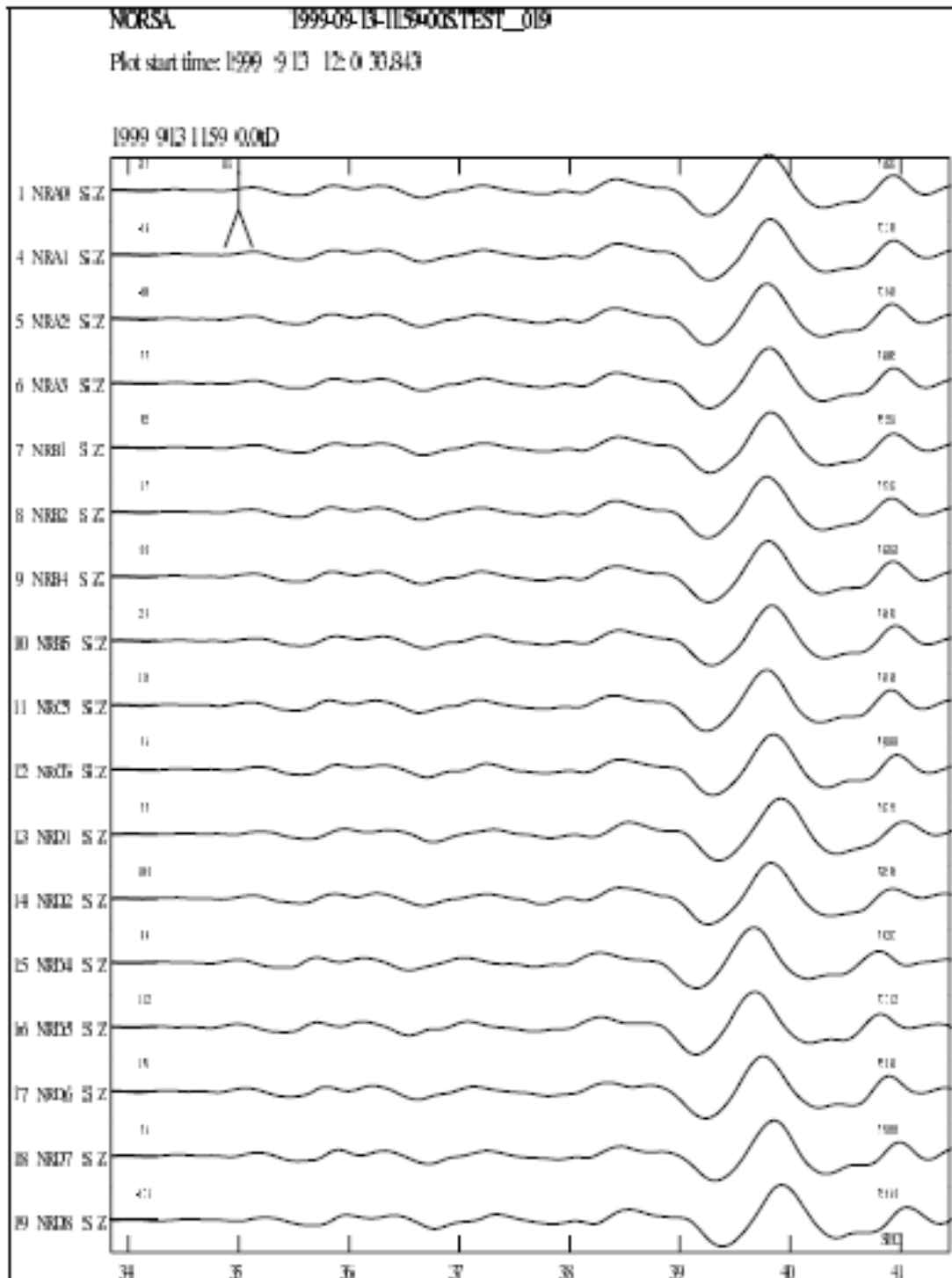
Figure 6.50: The FK program can be started from MULPLT. The traces shown were selected and used as input to the FK program. The result of the FK analysis is shown in Figure 6.51. The event shown here is part of the testdata set.
