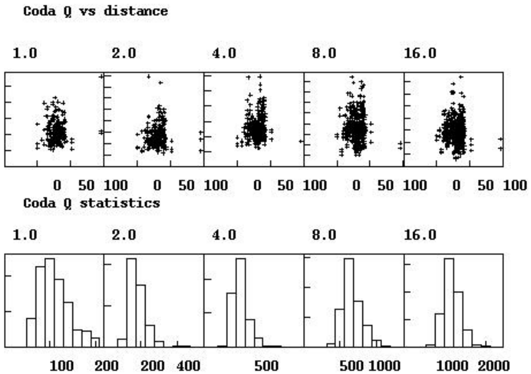
Figure 6.40: The top plot shows Coda Q as a function of epicentral distance and the bottom plot shows the distribution of individual Q-values for each frequency.
