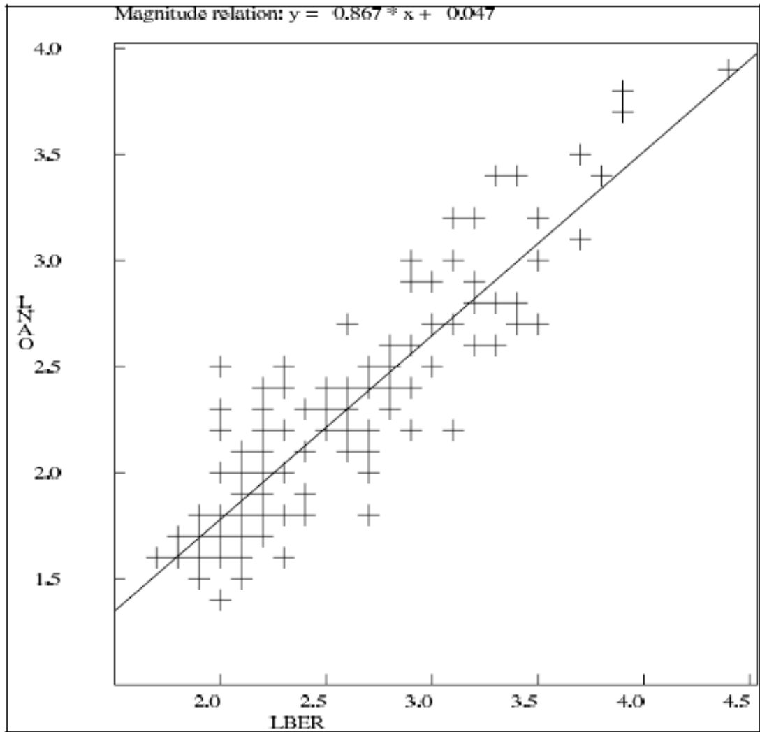
Figure 6.47: Example of using the MAG program. Relation between NORSEAR and Bergen local magnitudes.
