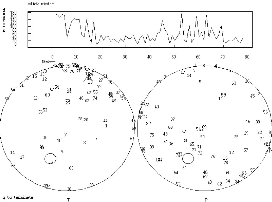
Figure 6.33: Left: The position of the T-axis given by the event numbers. The triangle is the SLICK minimum compressive stress direction and the circle is the null axis. Right: Corresponding for P-axis and the triangle is now the maximum compressive stress direction. Top: The misfit for each event as a function of event number. This figure can also show the cumulative misfit, see example run of FOC.
