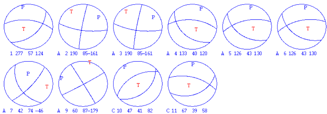
Figure 6.31: Example of plotting many solutions. Each solution is given with number, the fault plane solution and the quality (A-E). Up to 24 solutions can be plotted on one page.
