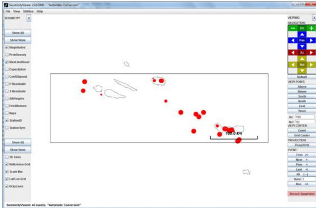
Figure 6.20: Epicenter map by SEIS2VIEWER.
