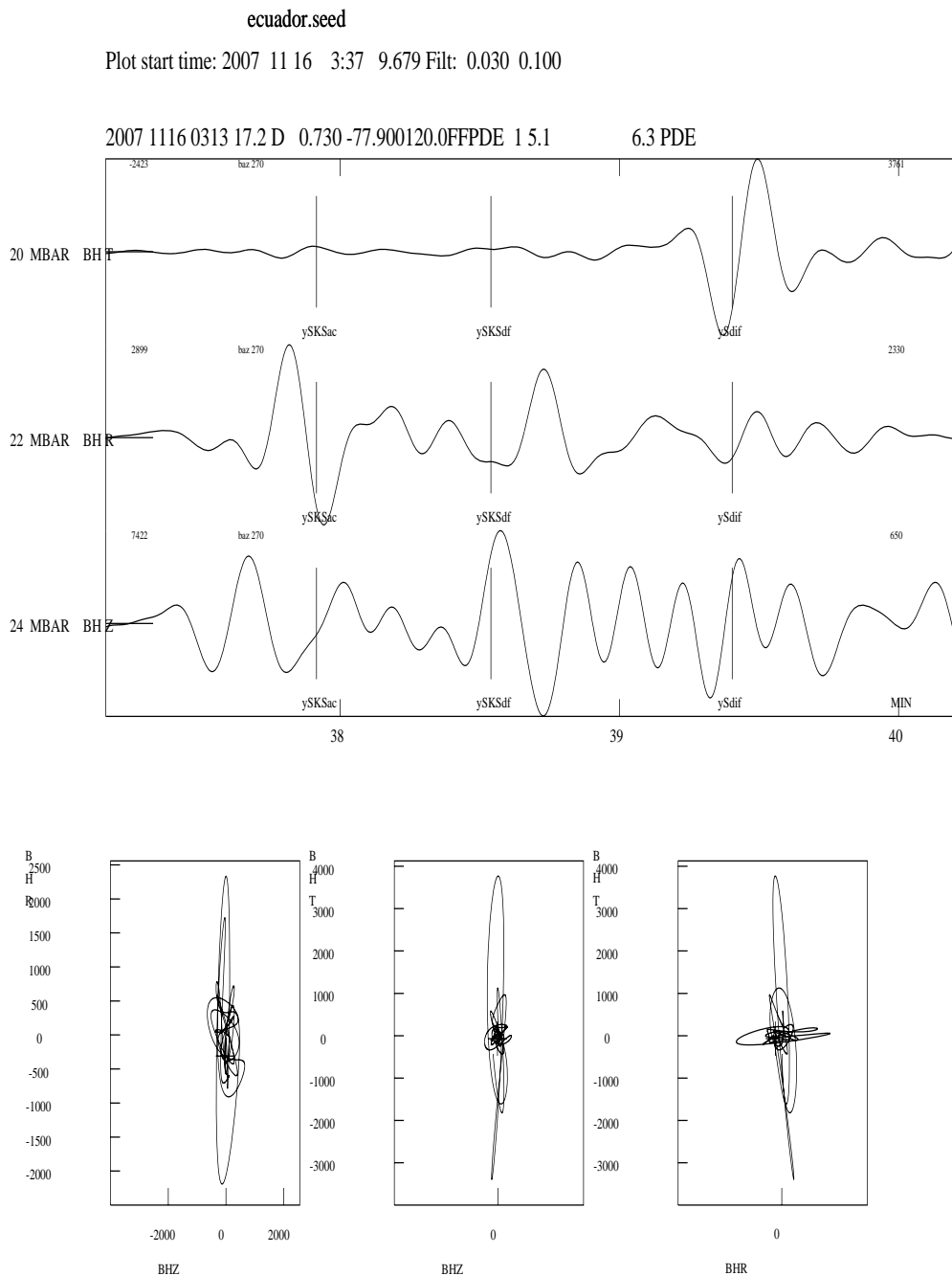
Figure 27 Example of particle motion plot.
