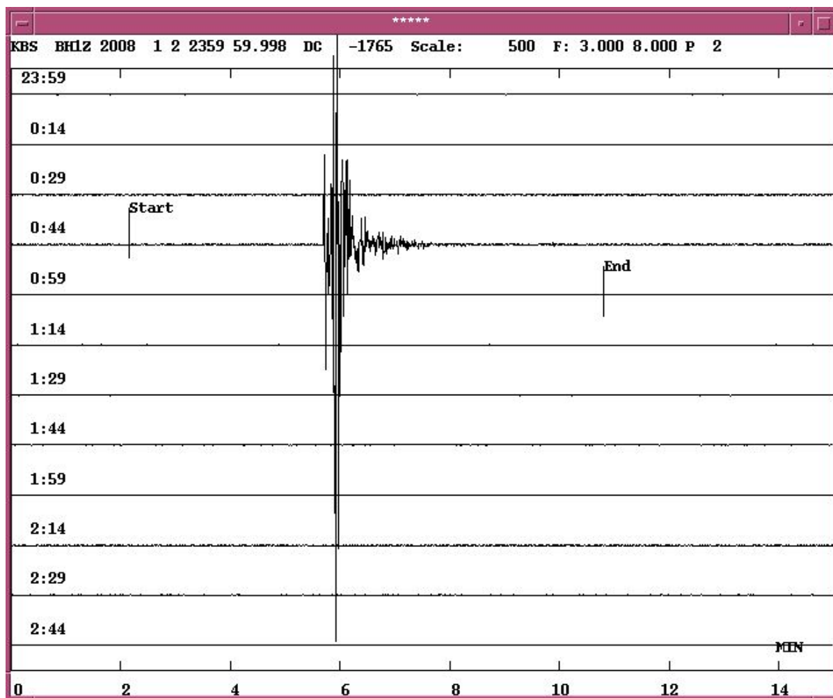
Figure 16. Example of time marks at the 'Start' and 'End' of an event recorded at the KBS station. The time marks is written to the file mulplt.ext for data to be extracted and processed. Type 's' and 'e' to add time marks.
