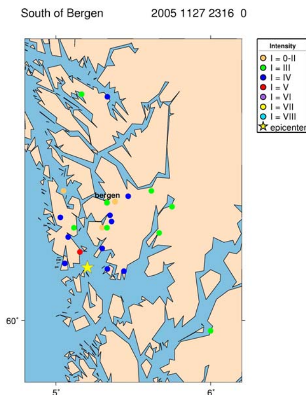
Figure 49 Macroseismic map made with MACROMAP using EEV. The epicenter, taken from the S-file, is shown with the star.
