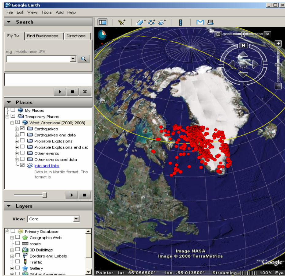
Figure 32 Example of mapping with gmap. Events in west Greenland . Note the folder and the subfolders in the “Places” window.
