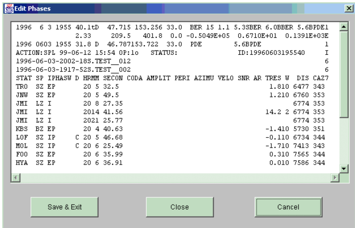
Figure 12. Editing window.
